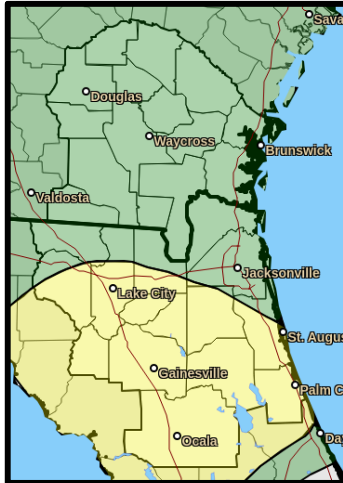
Probability of Excessive Rainfall (Tuesday)
