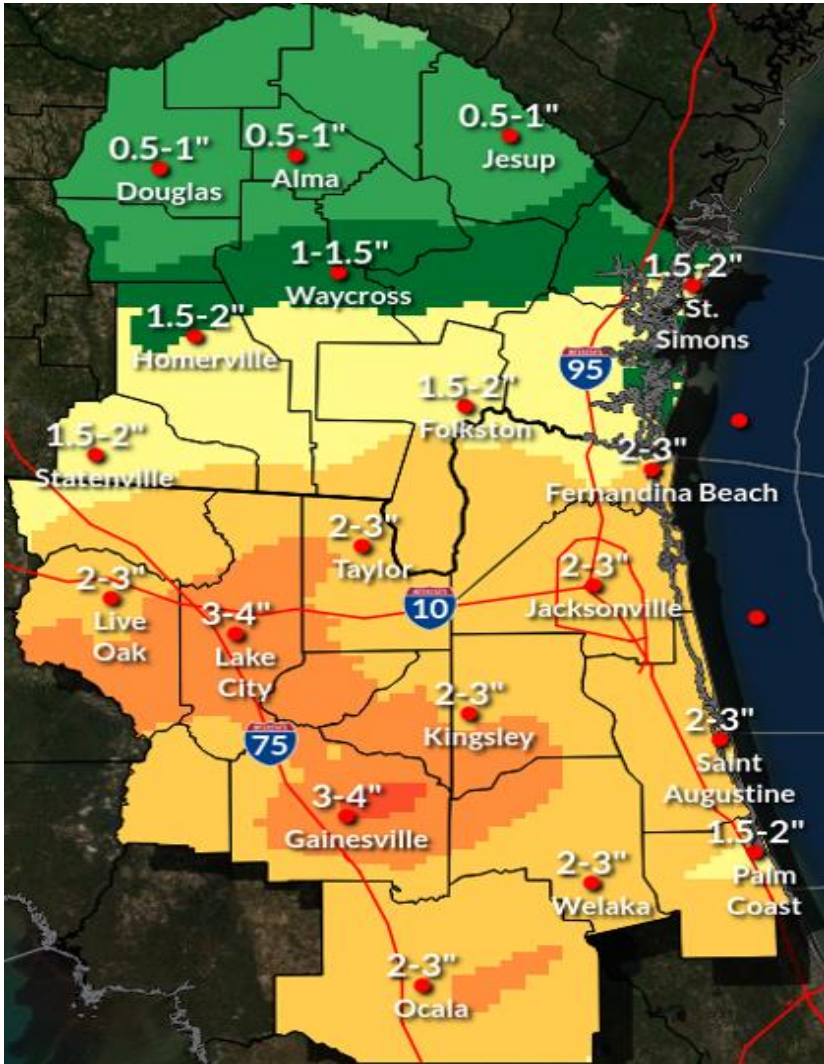
Official Storm Total Rainfall Forecast
