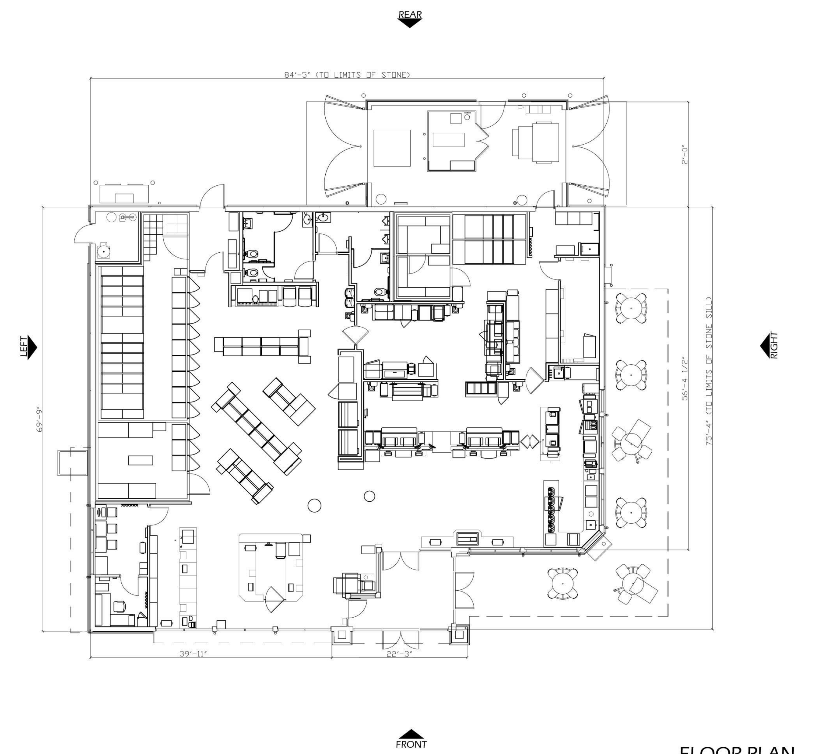
FLOOR PLAN
