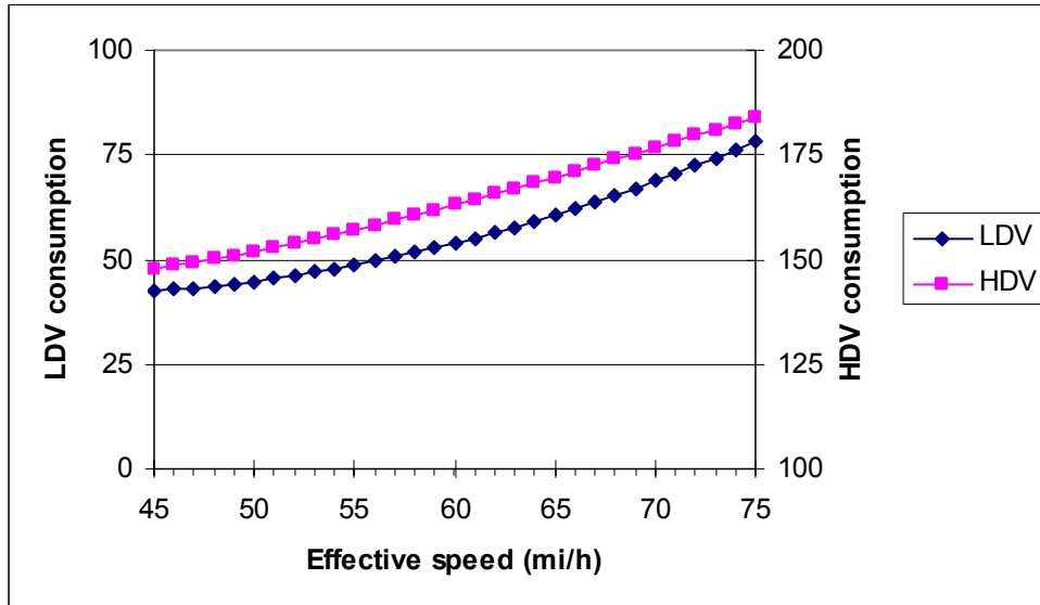
Figure 2-1 – Fuel Consumption at Constant Speed (gallons/1000 miles)
