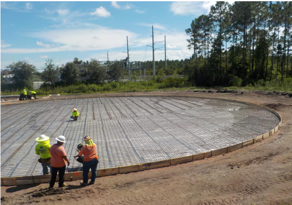
Waste Water Treatment Plant #2 Ground Storage Tank Rebar Matting for Foundation
